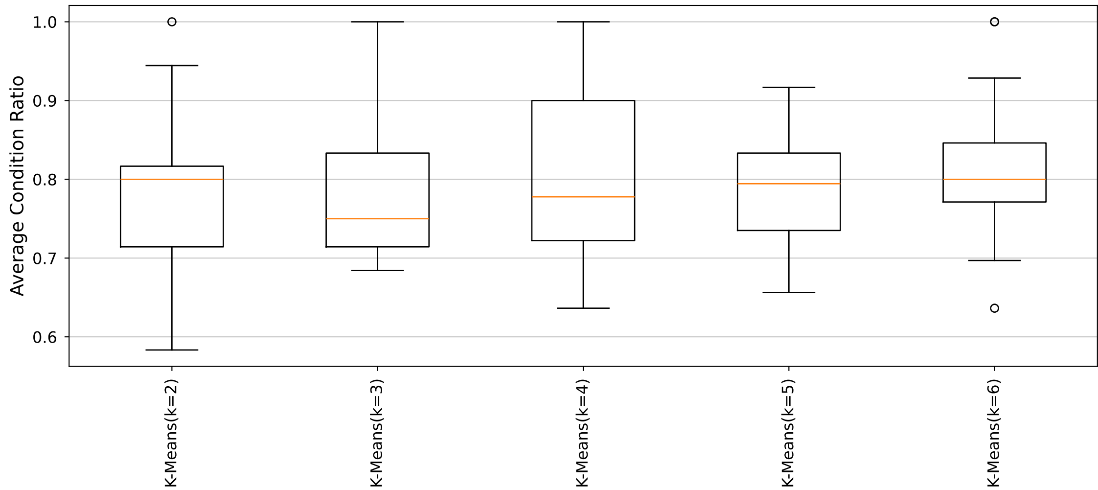
YARA Rules Average Condition Ratio Distribution (Cluster25_Size6 dataset)
